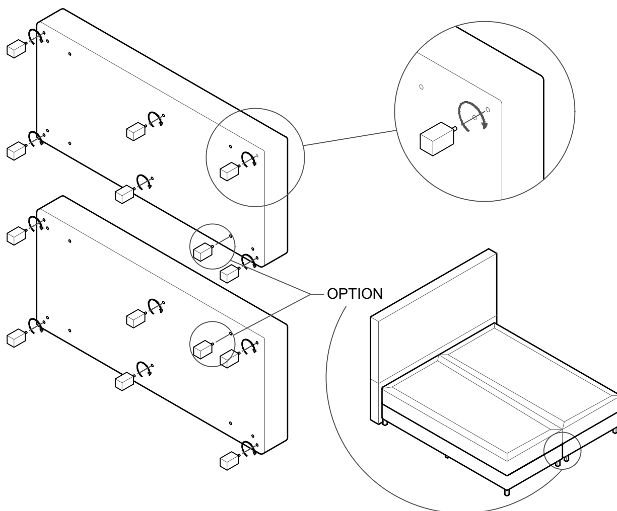
OPTION B BACK VIEW ASSEMBLY
