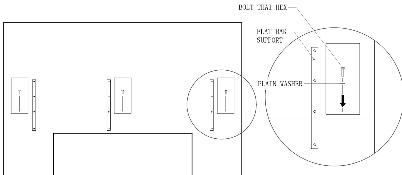
OPTION A BACK VIEW ASSEMBLY
