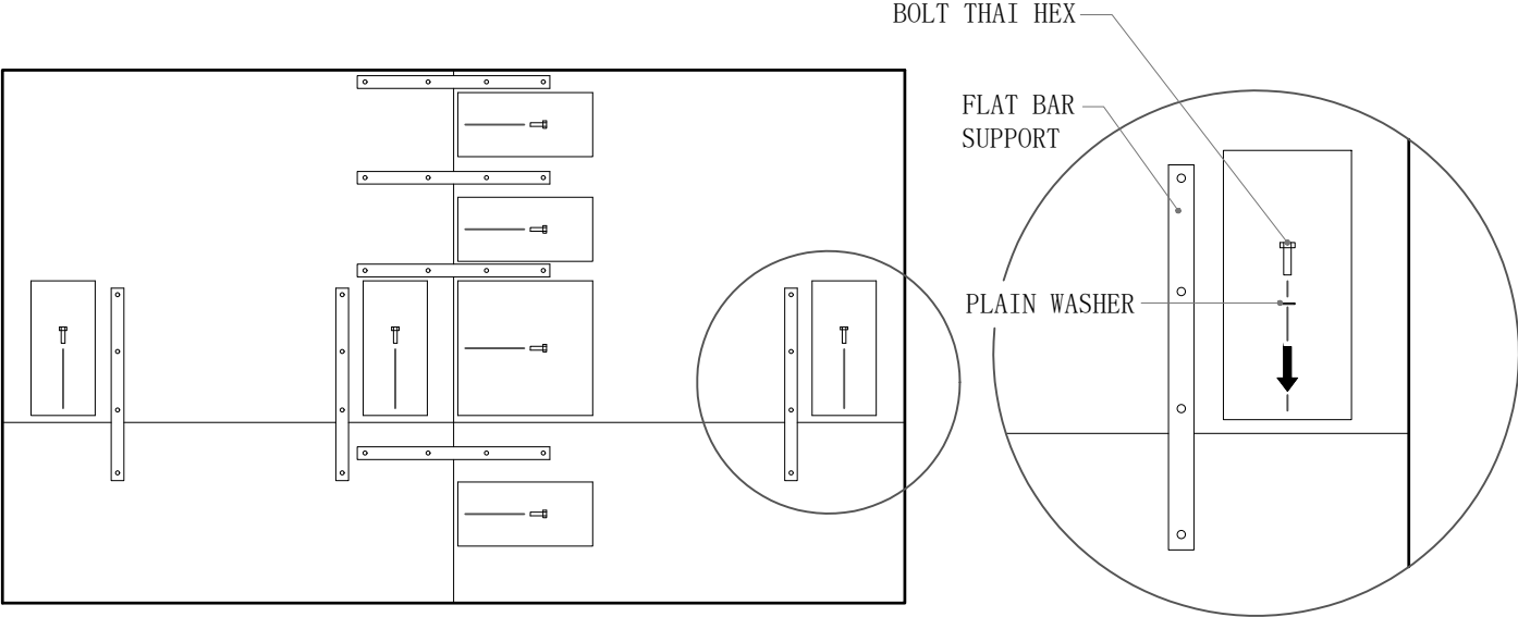
OPTION B BACK VIEW ASSEMBLY
